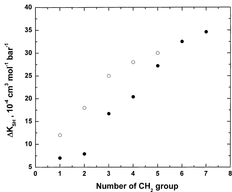
Fig. 5. The dependences on the number of -\text{CH}_2- groups of changes in adiabatic compressibility accompanying neutralization of carboxyl termini in \alpha, \omega -aminocarboxylic acids (this work (●)) and \alpha -carboxylic acids (from Ref. [27] (○)).
