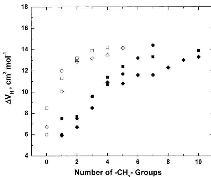
Fig. 2. The dependences on the number of -\text{CH}_2- groups of changes in volume accompanying neutralization of carboxyl termini in \alpha,\omega -aminocarboxylic acids (this work (●); Ref. [60] (■); and Ref. [61] (◆)), \alpha -carboxylic acids (Ref. [27] (□); and Ref. [62] (○)), and dicarboxylic acids (Ref. [28] (◇)).
