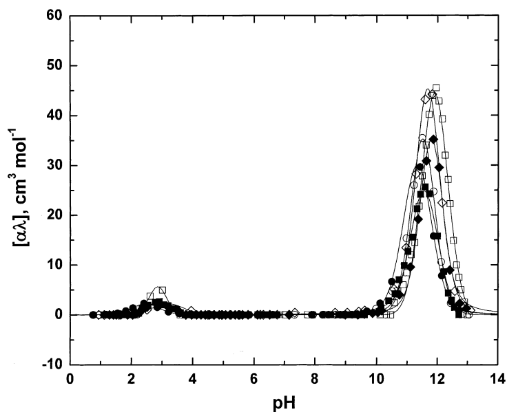
Fig. 4. The pH dependences of the molar increments of ultrasonic absorption per wavelength of \beta -alanine ( \bullet ), 4-aminobutanoic acid ( \circ ), 5-aminopentanoic acid ( \blacksquare ), 6-aminohexanoic acid ( \square ), 7-aminoheptanoic acid ( \blacklozenge ), and 8-aminooctanoic acid ( \diamond ). The fitting of the experimental data (solid lines) was accomplished using Eqs. (10), (10a), (10b), (10c) and (10d), as explained in text.
