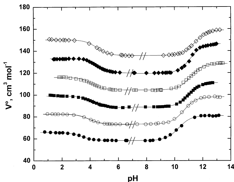
Fig. 1. The pH dependences of the partial molar volumes of \beta -alanine ( \bullet ), 4-aminobutanoic acid ( \circ ), 5-aminopentanoic acid ( \blacksquare ), 6-aminohexanoic acid ( \square ), 7-aminoheptanoic acid ( \blacklozenge ), and 8-aminooctanoic acid ( \diamond ). The fitting of the experimental data (solid lines) was accomplished using Eqs. (7a) and (7b), as explained in text.
