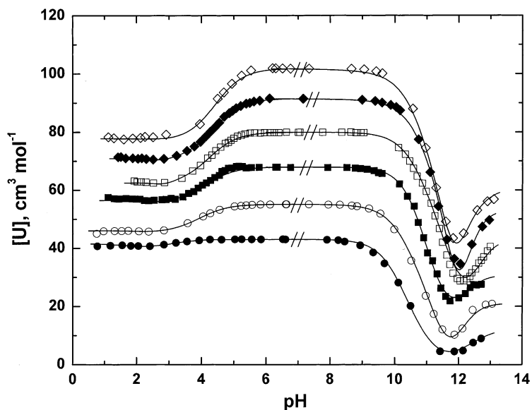
Fig. 3. The pH dependences of the relative molar sound velocity increments of \beta -alanine ( \bullet ), 4-aminobutanoic acid ( \circ ), 5-aminopentanoic acid ( \blacksquare ), 6-aminohexanoic acid ( \square ), 7-aminoheptanoic acid ( \blacklozenge ), and 8-aminooctanoic acid ( \diamond ). The fitting of the experimental data (solid lines) was accomplished using Eqs. (8), (9a), (9b), (10) and (11), as explained in text.
