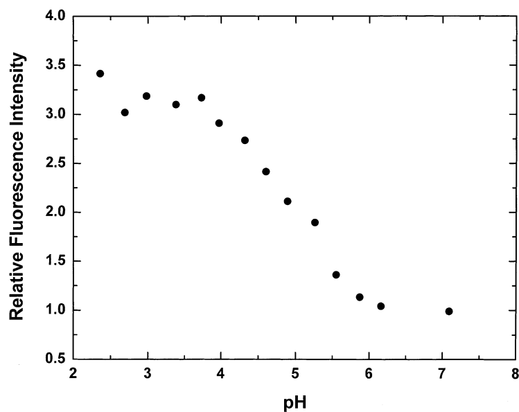
Fig. 6. The pH dependence of the differential fluorescence intensity of ANS in a solution of 8-amino-octanoic acid and water at 515 nm. The excitation wavelength is 370 nm.
